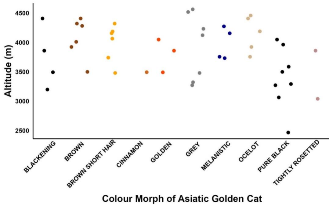
Fig. 4. Graph showing the altitude wise record of the different colour morphs of Asiatic golden cat.
