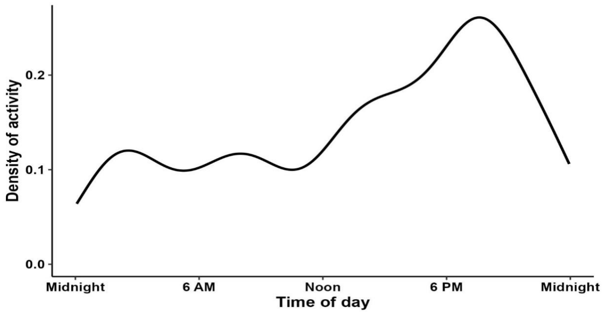
Fig. 2. Activity patterns of Asiatic golden cats in WCNP.
