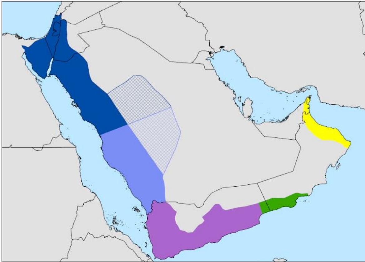
Fig SOM. Arabian leopard spatial units (Al Hikmani et al. 2025). Dark blue = North-west Arabia (Hijaz Mountains, Jordanian Highlands, An-Naqab / Negev desert, Sinai Peninsula); light blue = West Arabia (Asir Mountains); purple = South Arabia (Yemeni Highlands); green = South-east Arabia (Hawf Mountains and Dhofar Mountains); yellow = East Arabia (Al Hajar Mountains including Musandam Peninsula). Cross-hatched areas indicate areas with sparse historical evidence of the Arabian leopard.
