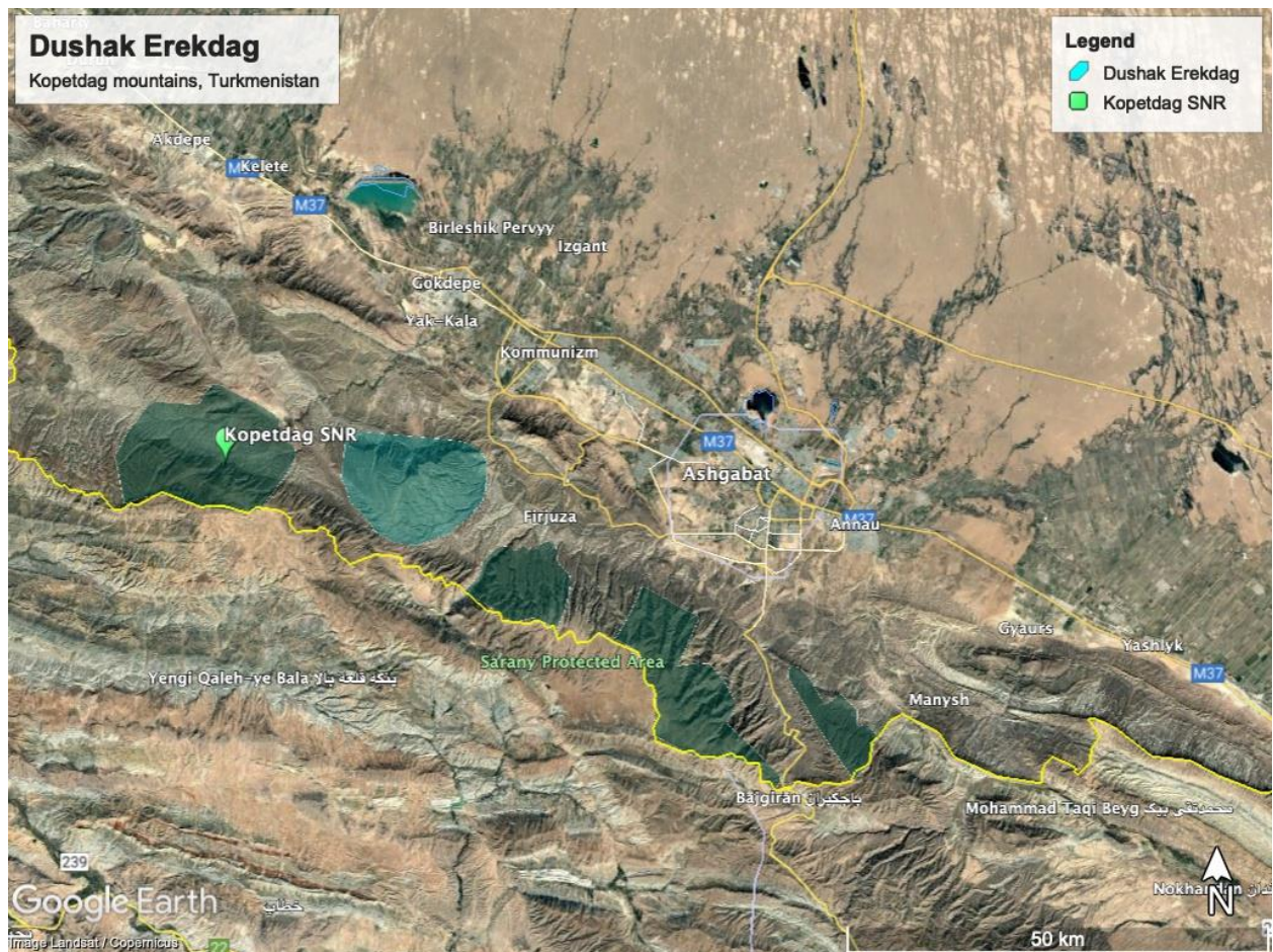
Fig. 1. Map of the Dushak Erekdag area in the Kopetdag mountains on the border between Turkmenistan and Iran.
