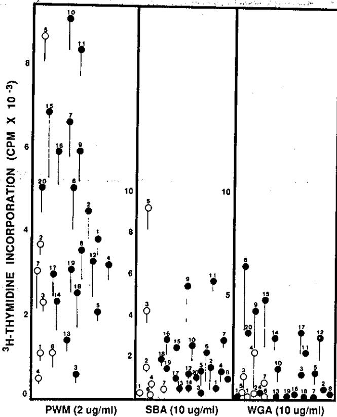
Fig. 2. Proliferative response of cheetah (solid symbols) and domestic cat (open symbols) PBM to 2 µg/ml PWM, 10 µg/ml SBA and 10 µg/ml WGA. See Fig. 1 for culture conditions and control values.
