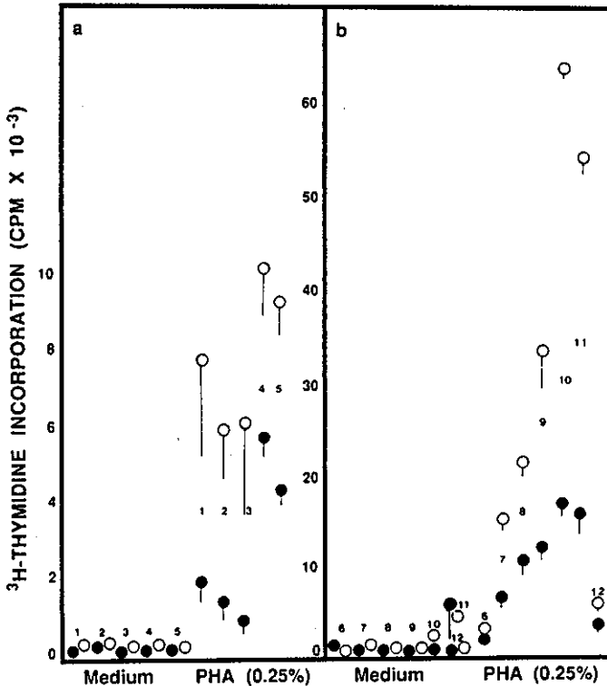
Fig. 3. Augmentation of PHA responses by exogenous IL-2. Cheetah PBM were stimulated with 0.25% PHA in the presence (open symbols) or absence (solid symbols) of exogenous IL-2 for 3 days. Mean values of 3 H-thymidine incorporation are expressed in cpm ± SD. Proliferation in unstimulated cultures with (open symbols) or without (solid symbols) exogenous IL-2 is also shown (medium). Panels (a) and (b) represent data from two groups of animals evaluated in separate experiments on different dates.
