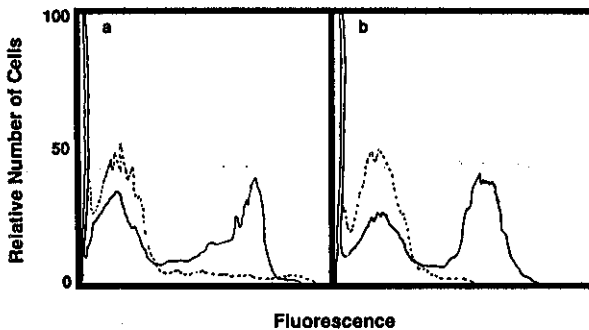
Fig. 4. Fluorescence intensity histograms of unstimulated domestic cat (a) and cheetah (b) PBM. Cells were stained with FT2 antibody and analyzed with a FACS (solid line). The dotted line corresponds to background staining; the X axis indicates fluorescence intensity (log 10 scale) and the Y axis shows relative numbers of cells.
